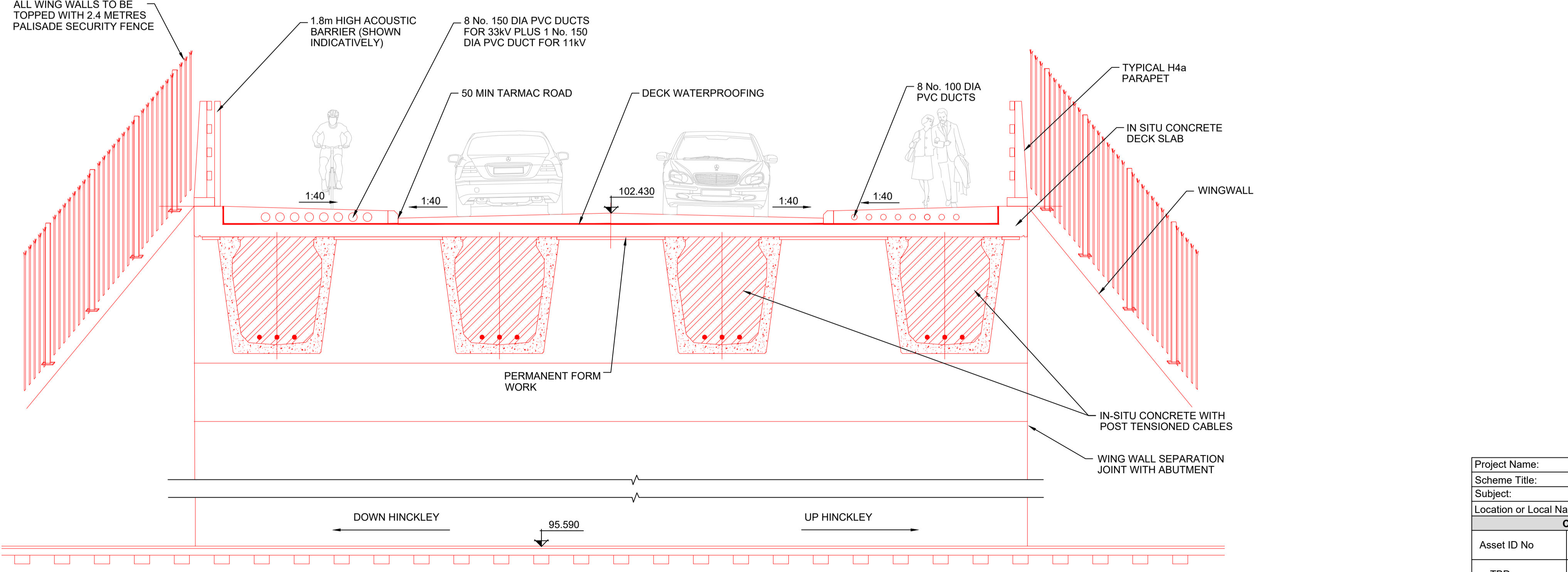
SECTION A TYPICAL CROSS SECTION SCALE 1:50
